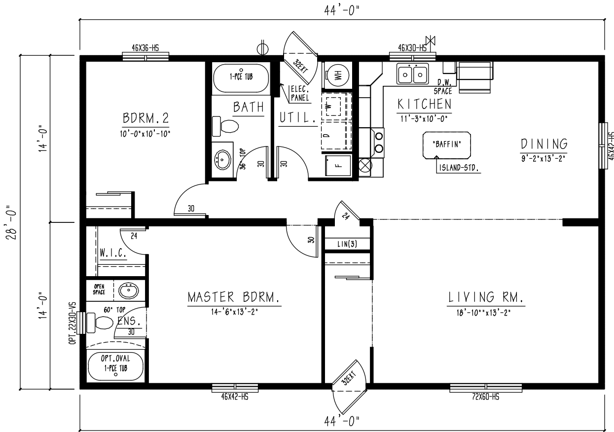
FLOOR PLAN SELF-CONTAINED [1232 SQ.FT.]
